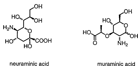
Figure 1. Naturally occurring ether amino acids
