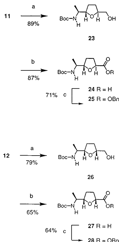
Scheme 5. Conversion of the THF alcohols 11 and 12 into the Boc-protected THF amino acid derivatives: (a) i: Na, NH 3 , -40°C, 10 min; ii: Boc 2 O, NaOH, MeOH; (b) i: dimethyl sulfoxide, oxalyl chloride, Et 3 N; ii: NaClO 2 , NaH 2 PO 4 , t BuOH; (c) BnBr, Et 3 N, acetone; Boc = tert -butoxycarbonyl
