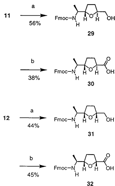
Scheme 6. Conversion of the THF alcohols 11 and 12 into the Fmoc-protected THF amino acid derivatives: (a) i: Na, NH_3 , -40^\circ C , 10 min; ii: Fmoc-succinimide, NaHCO_3 , MeCN/H_2O , 12 h room temp.; (b) i: dimethyl sulfoxide, oxalyl chloride, Et_3N ; ii: NaClO_2 , NaH_2PO_4 , tBuOH ; Fmoc = 9-fluorenylmethoxycarbonyl
