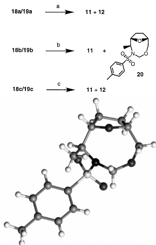
Scheme 3. Conversion of the diols 18 and 19 into the THF alcohols 11 and 12 : (a) i: NaH, tosylimidazole, THF; ii: 1 equiv. CSA, CH 2 Cl 2 , room temp., 2 h; (b) i: NaH, tosylimidazole, THF; ii: epoxide purification by column chromatography; iii: 0.1 equiv. CSA, CH 2 Cl 2 , room temp., 12 h; (c) i: NaH, tosylimidazole, THF; ii: HOAc/H 2 O 4:1, 40°C, 30 min; CSA = camphersulfonic acid
