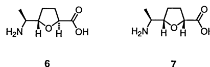
Figure 3. trans - and cis -THF amino acids 6 and 7
