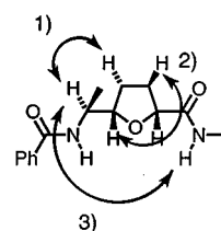
Figure 6. Selected NOESY crosspeaks found for 34 in \text{CDCl}_3 and used as input for the MD calculations
