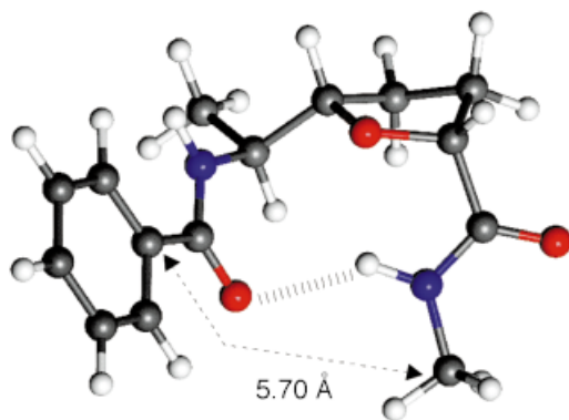
Figure 5. A: general \beta -turn structure; B: solid-state conformation of the cis -THF dipeptide 34 obtained by X-ray structural analysis; C: solution conformation ( \text{CDCl}_3 ) of the cis -THF dipeptide 34 obtained by NMR studies and MD calculations
