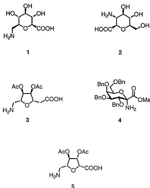
Figure 2. Sugar-derived synthetic THF and THF amino acids
