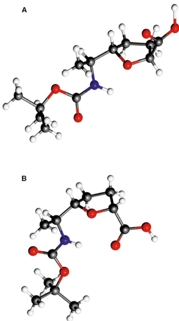
Figure 4. A: solid-state conformation of the trans -THF amino acid derivative 24 obtained by X-ray crystal-structural analysis; B: solid-state conformation of the cis -THF amino acid derivative 27 obtained by X-ray crystal-structural analysis
