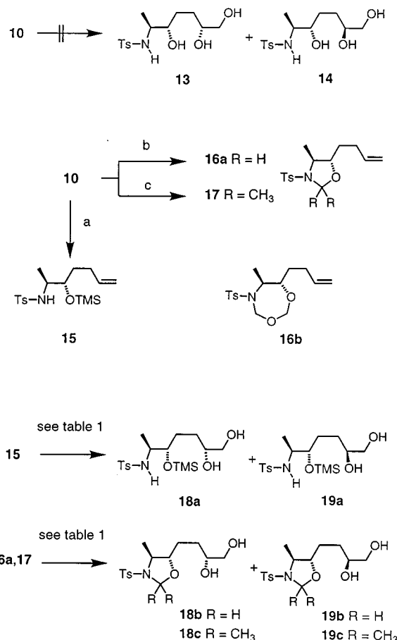
Scheme 2. Preparation of the alkenes 15 , 16a , and 17 and asymmetric dihydroxylation into the diols 18 and 19 : (a) \text{TMSCl} , \text{Et}_3\text{N} , \text{CH}_2\text{Cl}_2 , 94%; (b) paraformaldehyde, CSA, toluene, Dean–Stark trap, 65% 16a and 32% 16b ; treatment of 16b with CSA in \text{CH}_2\text{Cl}_2 afforded 16a in 98% yield; (c) 2,2-dimethoxypropane, CSA, room temp., 2 h, 92%; CSA = camphersulfonic acid
