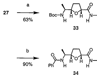
Scheme 7. Synthesis of the THF diamide 34 : (a) MeNH_2 \cdot HCl , EDC, HOBT, EtNIPr_2 , THF, room temp., 18 h; (b) i: TFA, CH_2Cl_2 , room temp., 4 h; ii: PhCOCl , NaHCO_3 , THF/H_2O , room temp., 1 h; EDC = N -(3-dimethylaminopropyl)- N' -ethylcarbodiimide, HOBT = 1-hydroxy-1 H -benzotriazole, TFA = trifluoroacetic acid
