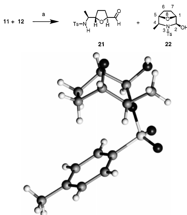
Scheme 4. Oxidation of a 1:1 mixture of the THF alcohols 11 and 12 : (a) Dess–Martin oxidation, 40% 21 and 40% 22 ; Swern oxidation, 31% 21 and 66% 22 ; X-ray structure of 22
